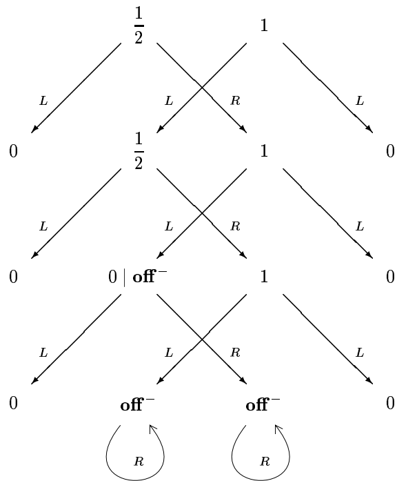
Figure 3: Computing G^- .
