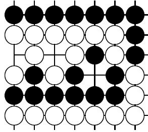
Figure 14: Triple ko.
