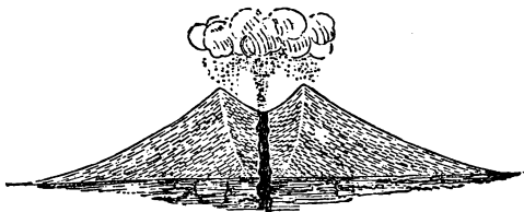
FIG. 51.—Diagrammatic Section of a Cinder Cone
