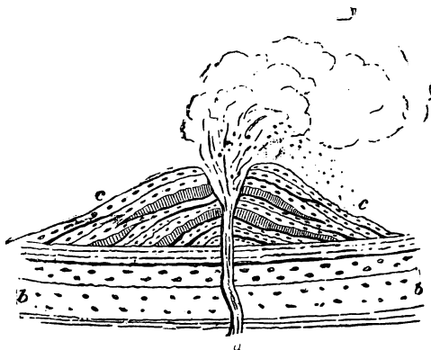
FIG. 50.—Diagrammatic Section of a Volcano
