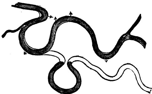
Diagram Showing the Wanderings of a Stream in an Alluvial Plain
